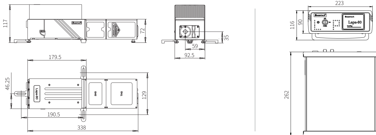
Lapa-80/100 激光头
